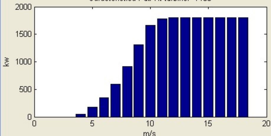
Caracteristica Put/Vit turbinei V100
