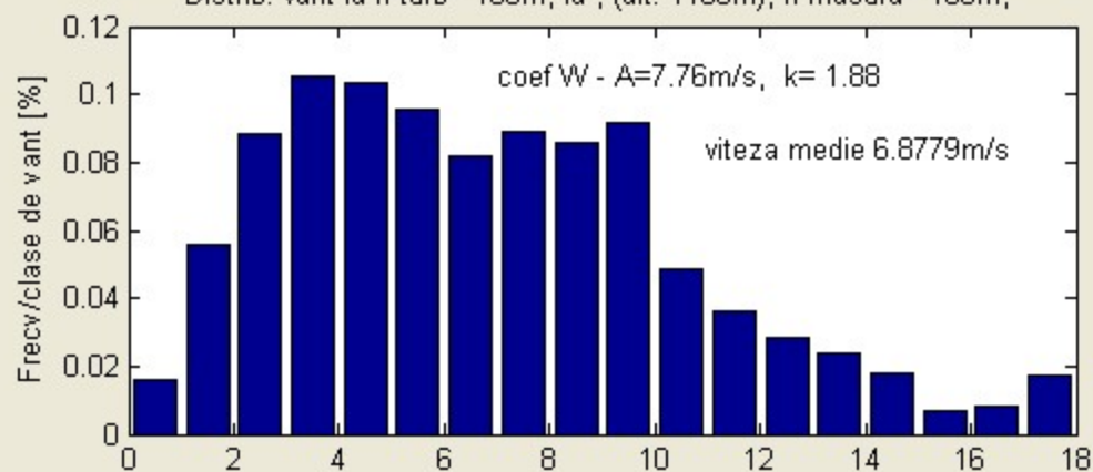
Distrib. vant la h turb= 100m, la , (alt. 1100m), h masura= 100m,
